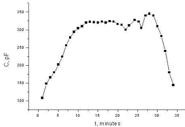
Fig. 5. Capacity of the 50%-aqueous solution of alcohol affected by the TC as a function of time at the frequency of measuring electric field f_{\text{meas}} = 100 Hz.
